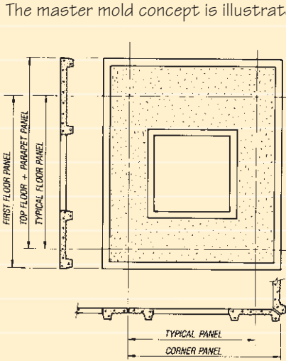
Fig. 1C—Three views of a master mold.
