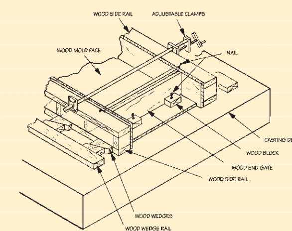
Fig. 1E—Removable sections within a master mold.
